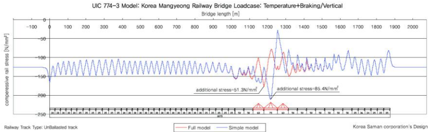
Figure 3. Compressive stress in the rails from temperature and braking loading for Mangyeong River Crossing, Honam High Speed Railway, South Korea.
