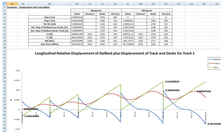
Figure 2. Envelope of axial stresses in a rail track from temperature loading
