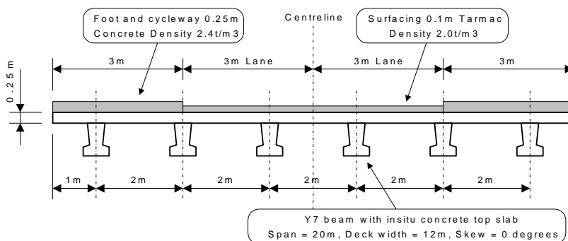
Cross-section through deck
