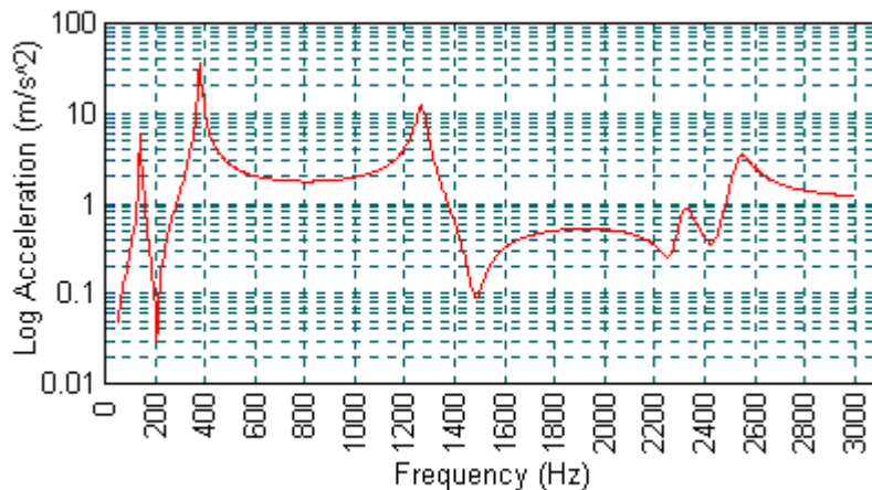
FRF in Z Direction at Centre of Back Plate (2.8% Structural Damping)
