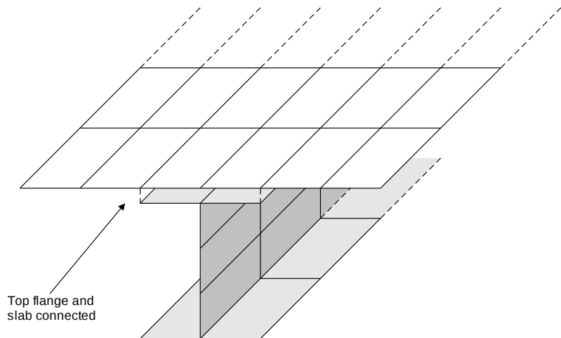
Shell element modelling of the whole structure
