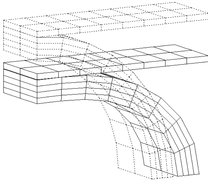
Figure 1: Deformation of cylinder at increment 36
