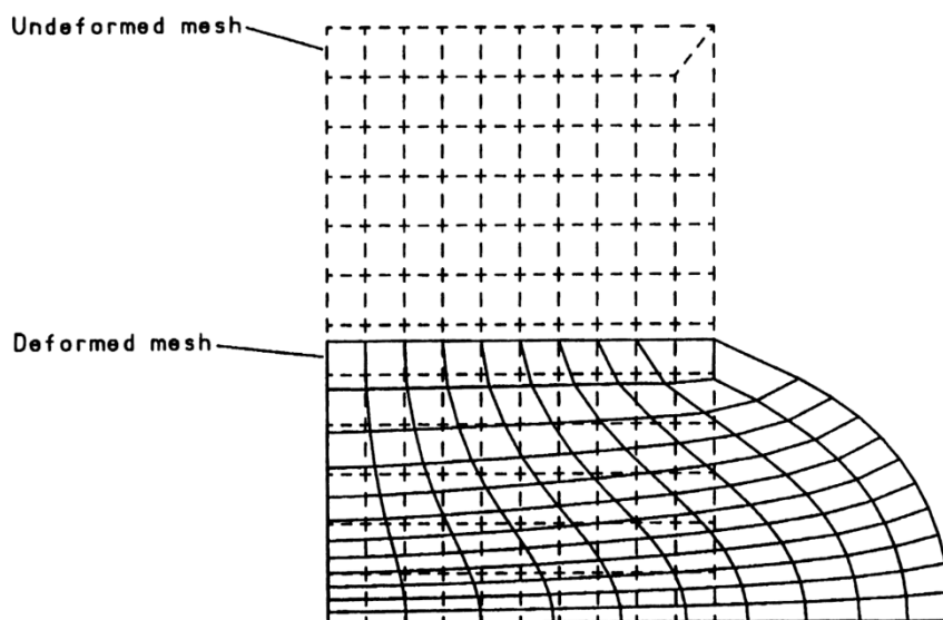
Figure 1. Deformed mesh plot at 52% upsetting
