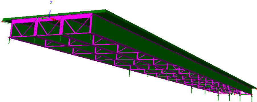
Straight multi-span steel composite bridge deck with bracing created by the wizard
