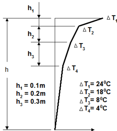
Reproduction of EN1991-1-5:2003 Figure 6.2a.
