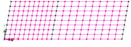
Multiple span skewed slab deck
