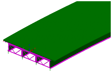
Fleshed view showing beam and shell elements used
