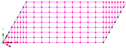
Single span orthogonal slab deck
