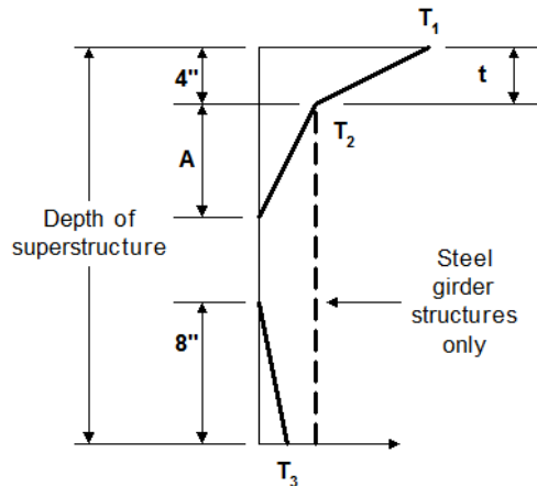
Reproduction of AASHTO 8th Fig 3.12.3-2
