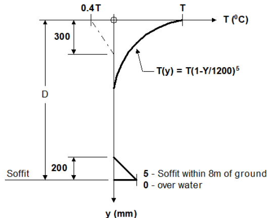
Reproduction of AS 5100 Figure 18.3
