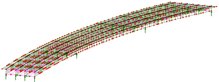
Span lines (highlighted in black) created at bridge deck level defining four composite design members
