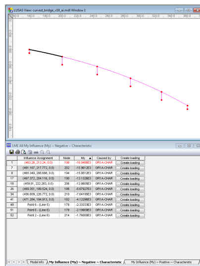
Influence results filtered to show only those results for a selected feature (span 5)
