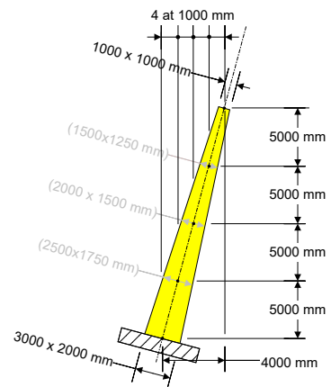
Tower geometry and construction stages
