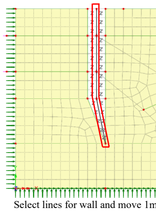
Figure 61: Close gap between wall and soil
