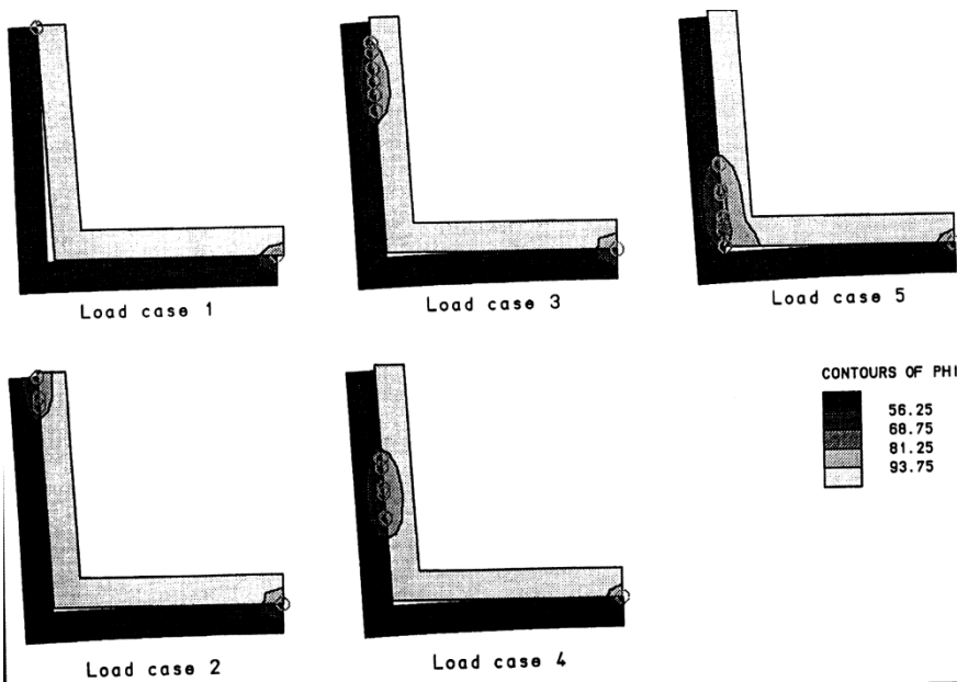
Figure 4 Temperature contours and contact points (circled)
