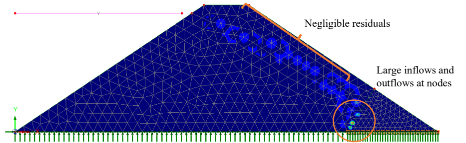
Figure 6: Flow residuals for the simple parameters
