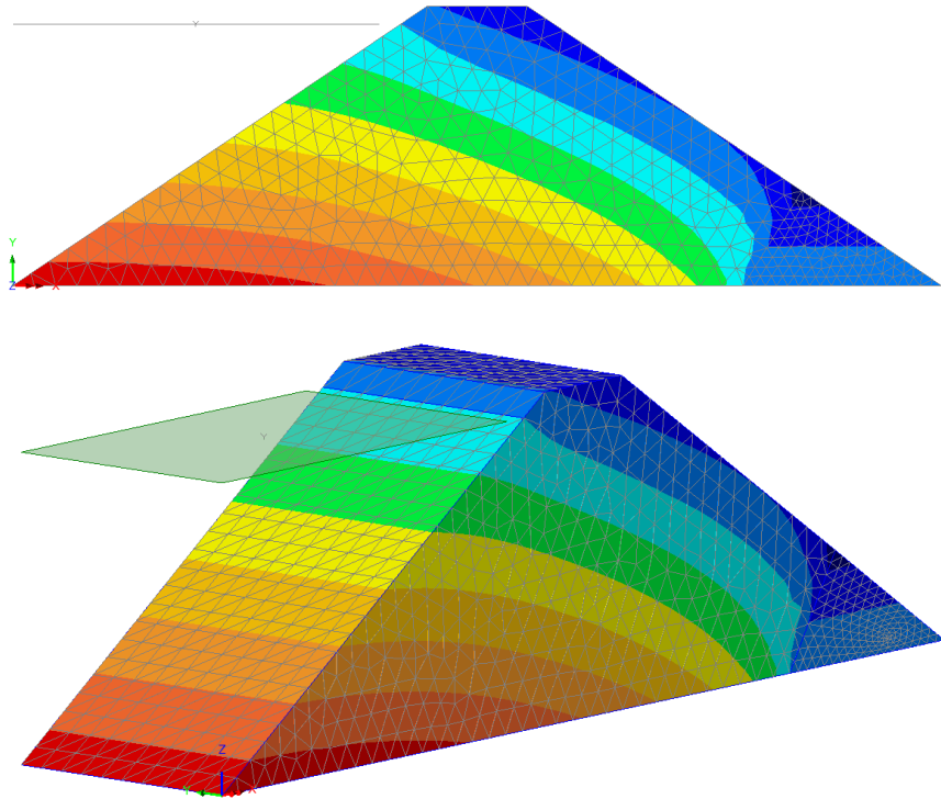
Figure 7. Pressure contour plots for 2 and 3D solutions
