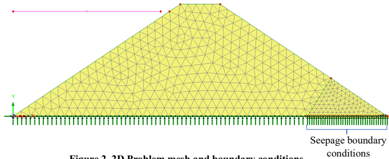
Figure 2. 2D Problem mesh and boundary conditions
