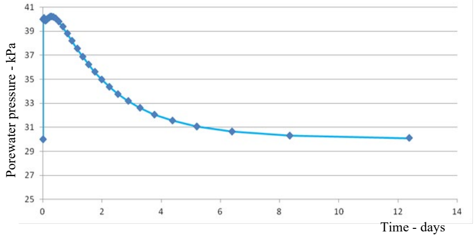
Figure 2.16.1 Typical change of porewater pressure during consolidation
