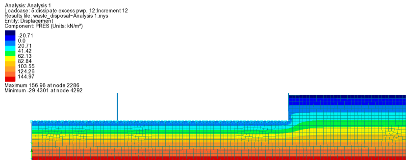
Figure 16: Steady state pore water distribution
