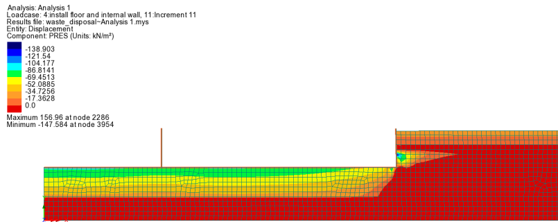
Figure 15: Suction pressure after installation of floor slab and partition wall
