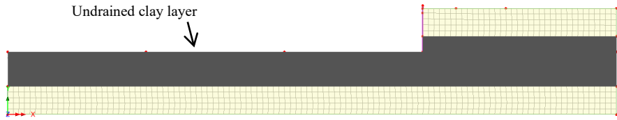
Figure 5: Undrained excavation
