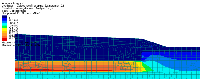
Figure 17: Excess pore water pressure at end of loading
