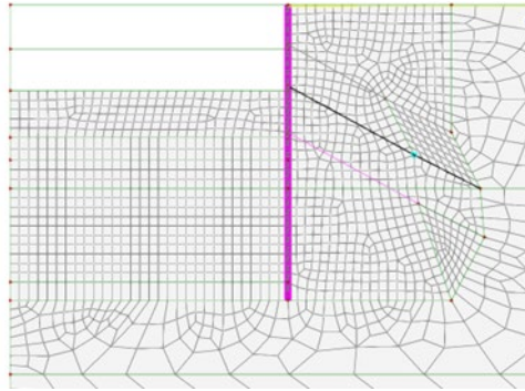
Figure 22: Installing second row anchors
