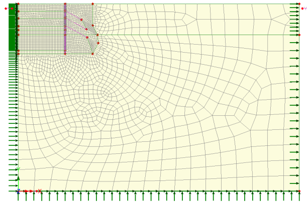
Figure 9: Boundary conditions
