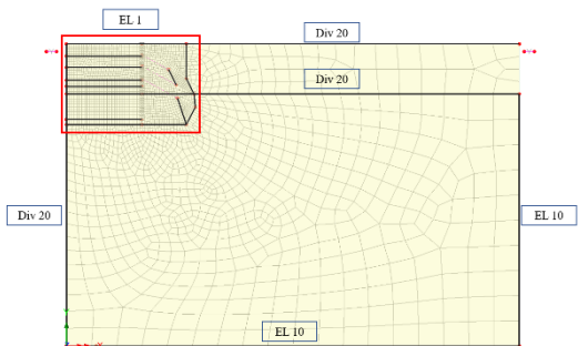
Figure 6: Model meshing
