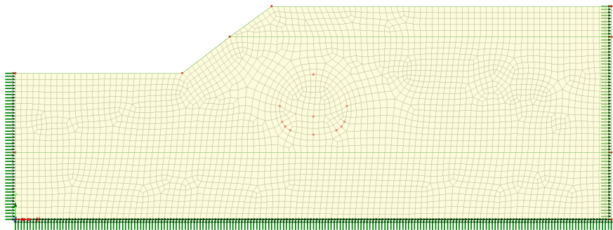
Figure 2. 2D Problem geometry and mesh
