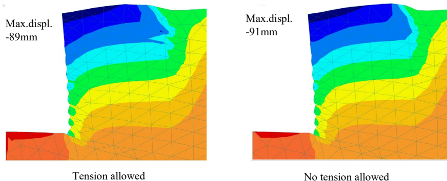
Figure 9: Horizontal displacements after installing final nail
