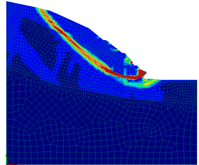
Effective shear strain
