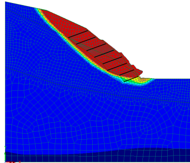
Deformed mesh at final stage of safety factor calculation
