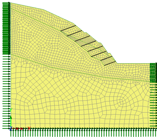
Figure 5: Model mesh with boundary conditions
