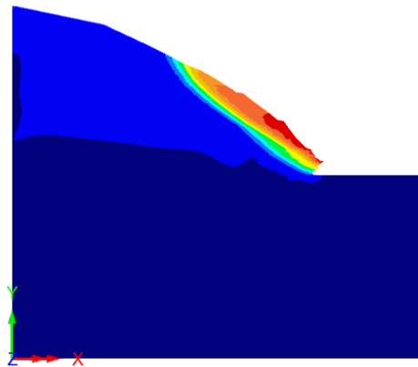
Figure 9: Results obtained based on Phi-c reduction calculation (no nails)
