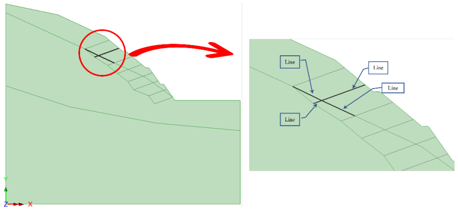
Figure 2: Decomposition of the model
