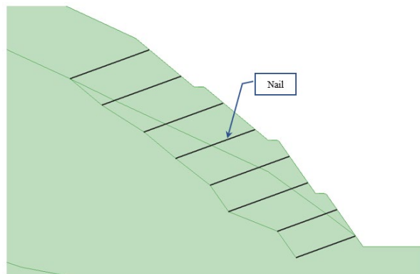
Figure 3: Slope stabilization using nails
