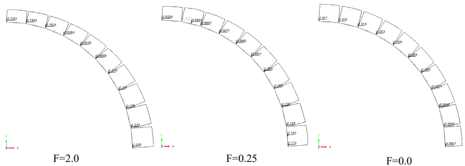
Figure 6: Distribution of normal stress
