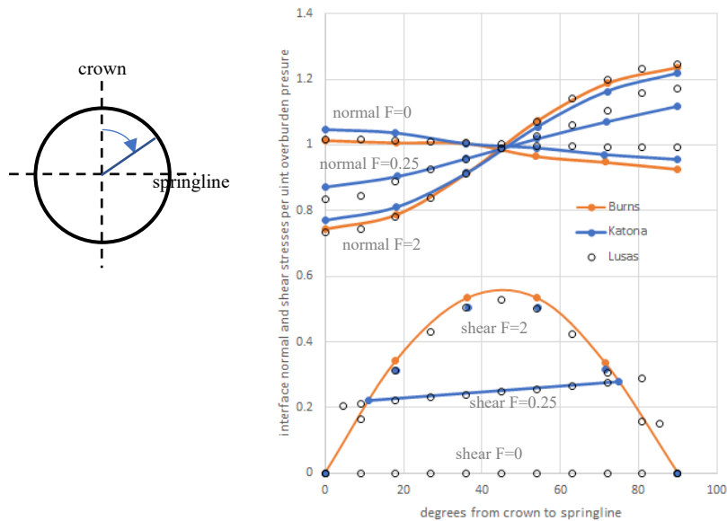
Figure 4: Variation of normal and shear stresses around pipe periphery
