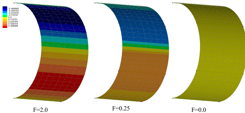
Figure 8: Contours of shear stress on interface of 3D model
