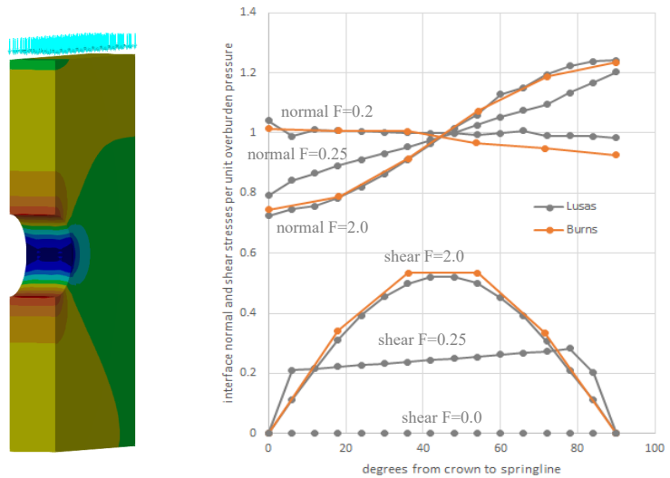
Figure 7: Results for 3D analysis
