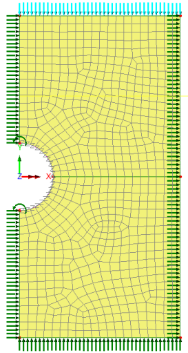
Figure 2: Finite element mesh showing supports and load
