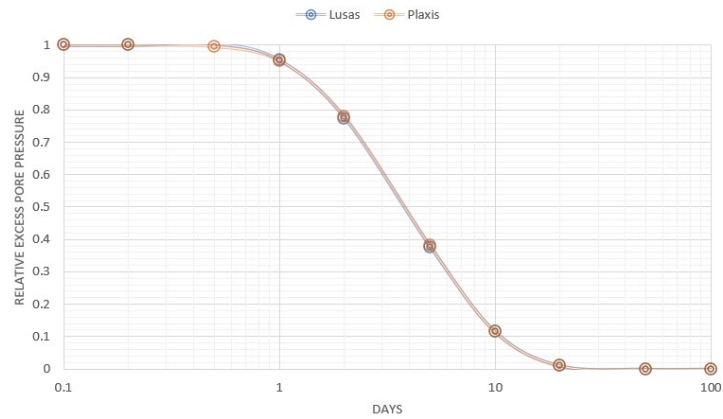
Figure 2: Comparison of pore pressure dissipation with time (LUSAS, PLAXIS)
