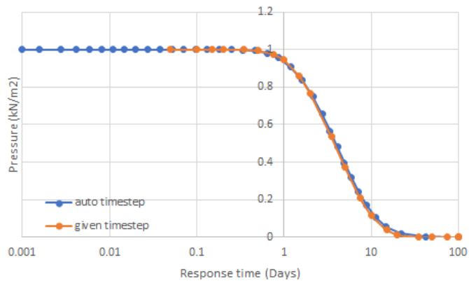
Figure 3: Comparison of given and automatic timestep solutions
