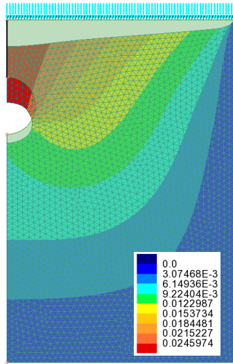
Figure 3: Displacement contours (m)
