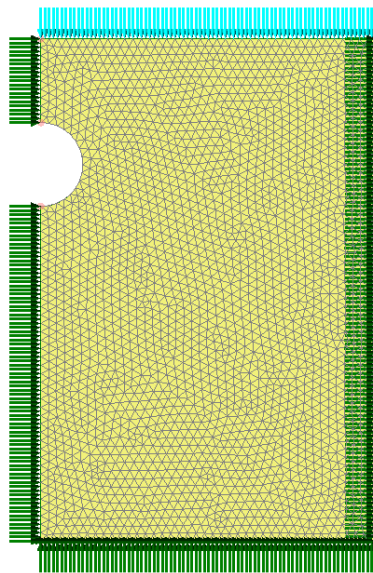
Figure 1: Finite element mesh showing supports.
