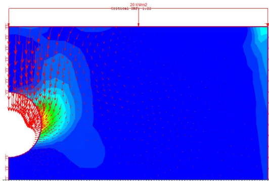
Figure 5: Maximum Shear Strain in RS2 [2]
