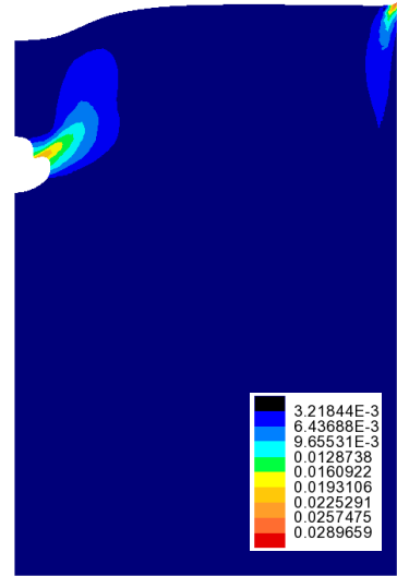
Figure 4: Maximum Shear Strain
