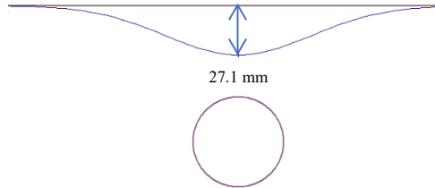
Figure 2: Maximum Settlement using analytical approach
