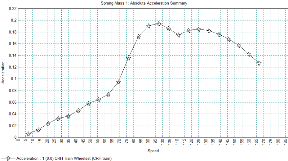
(First spring-mass system)
