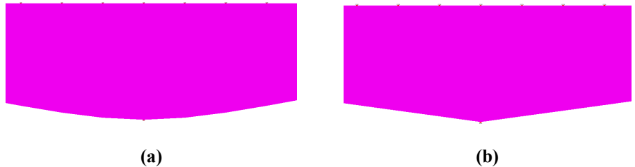
Figure 33: Zoomed Plot of Pier Location between Spans of Deck 1 Showing (a) Smoothed Section for a Multiple Varying Sections with One Reference Path per Deck and (b) Correct Unsmoothed Section for a Multiple Varying Sections with One Reference Path per Span
