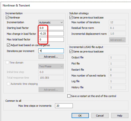
Load parameters for ramping down
