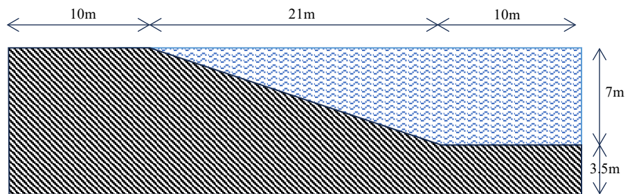
Model geometry
