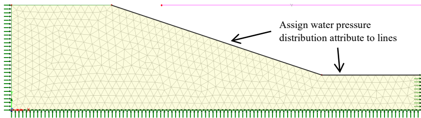
Assignment of water pressure distribution attribute
