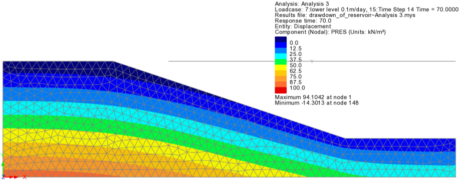
Day 70: Slow drawdown 0.1m/day
