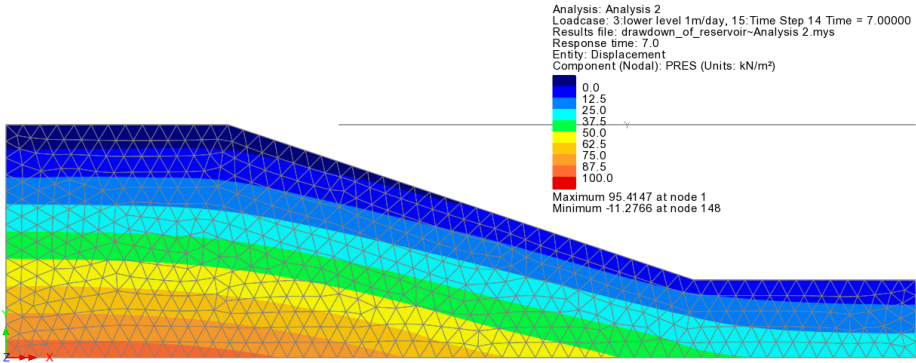
Day 7: Fast drawdown 1m/day
