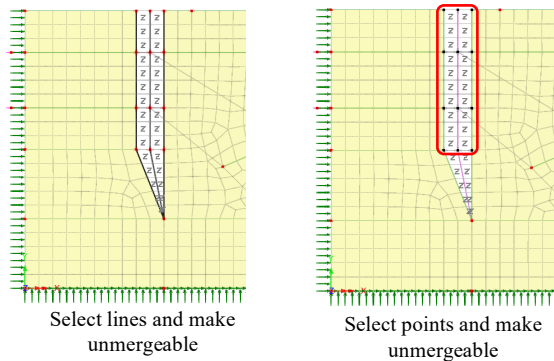
Figure 60: Make all geometry unmergeable before moving into place
