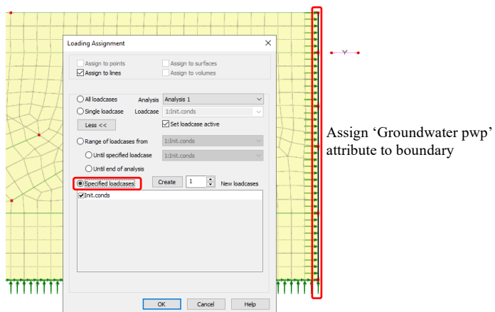
Figure 42: Setting groundwater conditions
